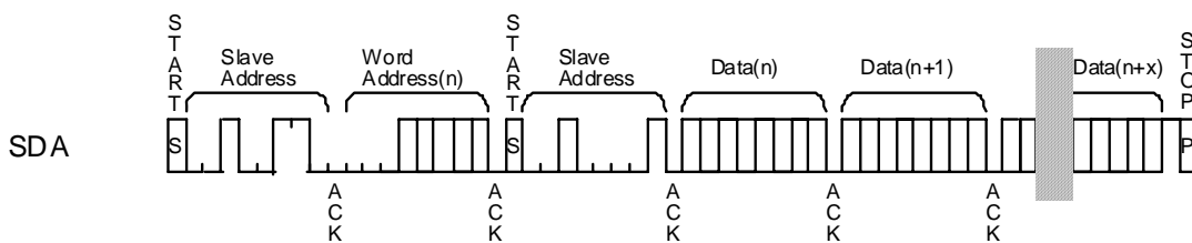
Figure 15. RANDOM READ
