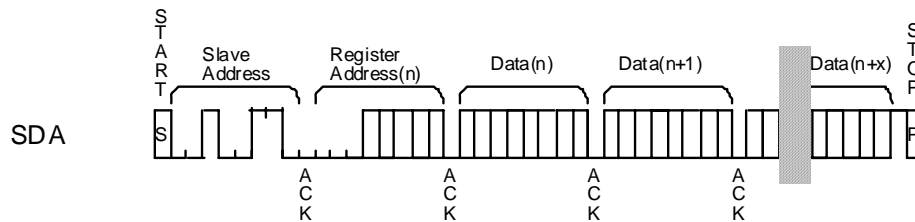
Figure 13. WRITE Operation
