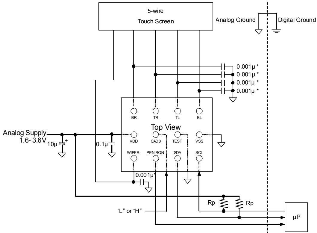
Figure 36. Typical Connection Diagram
