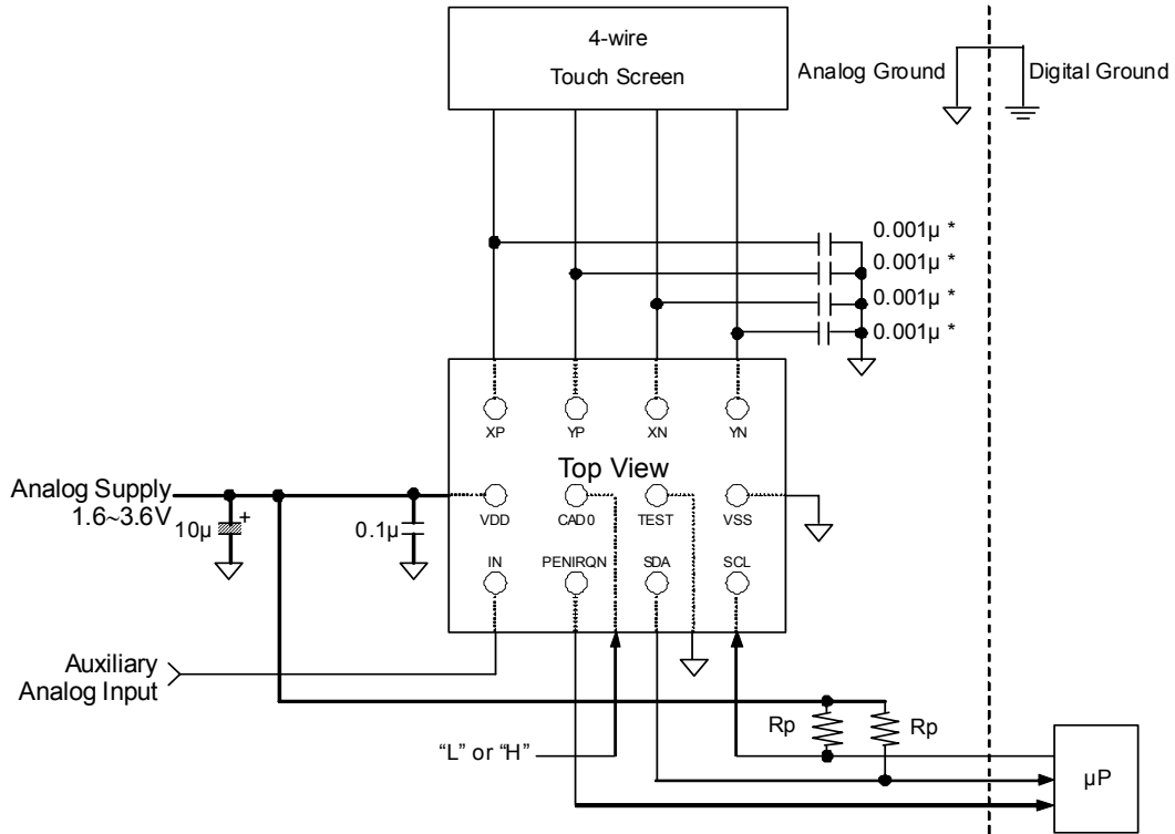
Figure 35. Typical Connection Diagram
