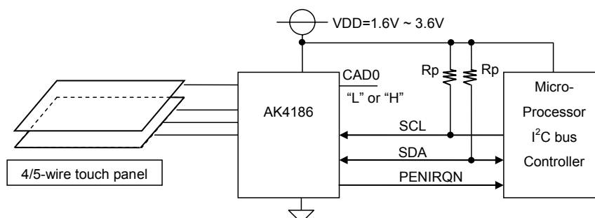
Figure 6. Digital I/F
